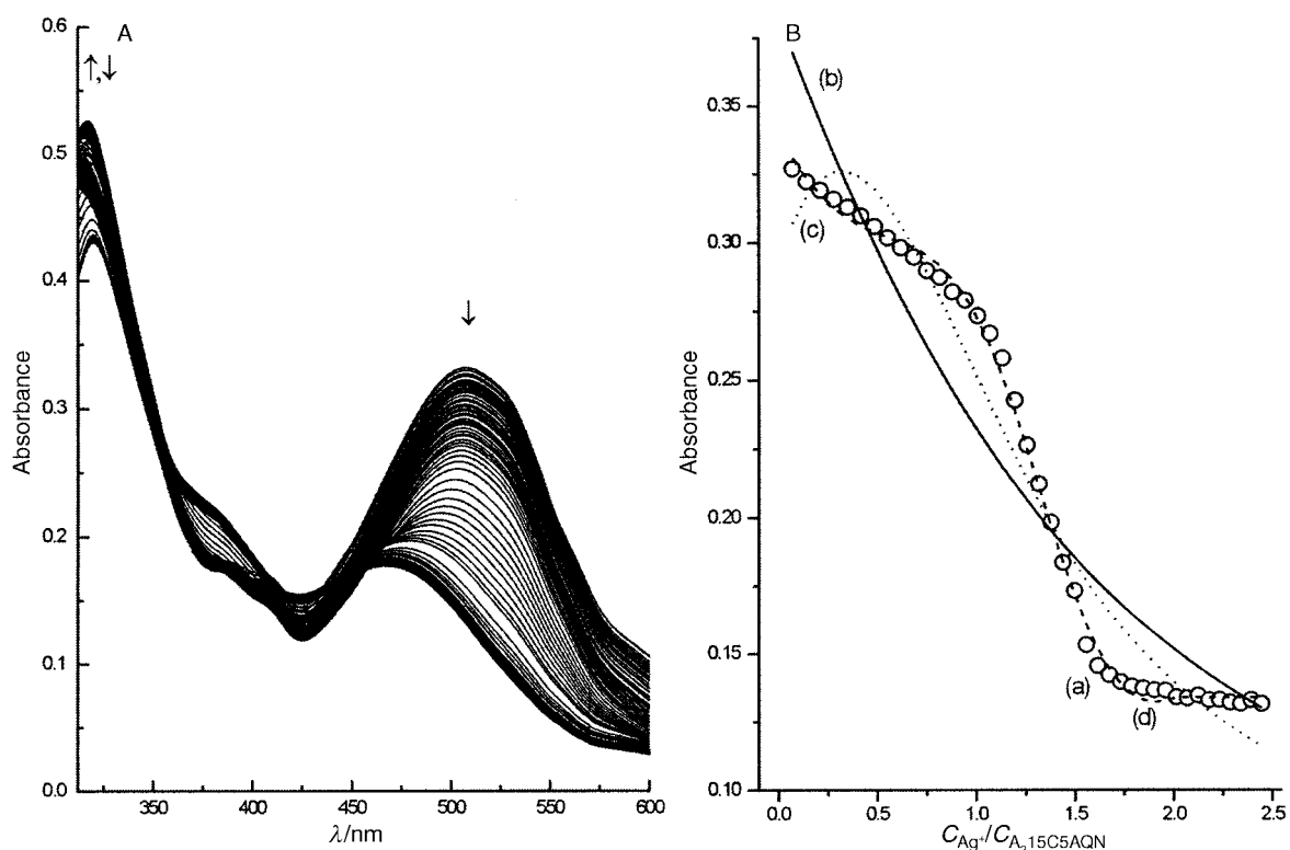
Fig. 4 A, Absorption spectra recorded in PC solutions containing A215C5AQN 8 ( 1.20 \times 10^{-4} \text{ mol dm}^{-3} ) and concentration of silver(I) perchlorate ( 0-6.00 \times 10^{-4} \text{ mol dm}^{-3} ). B, Dependence of absorbance at 510 nm for A215C5AQN 8 with silver perchlorate. The experimental points are (a) (open circles) and the fitting curves for the models are 1 (b) (line), 4 (c) (dotted line), 8 (d) (dashed line).
