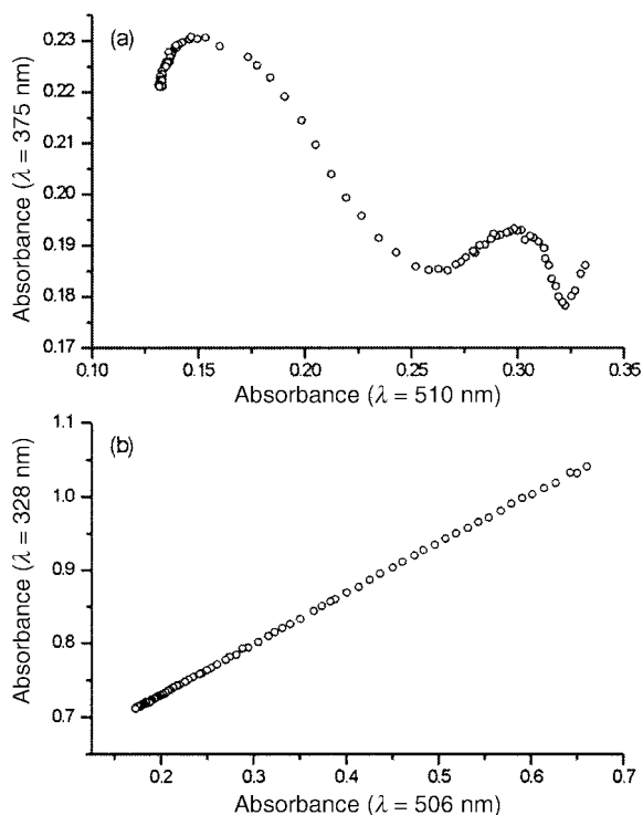
Fig. 5 Absorbance-absorbance diagrams for measurements of \text{A}_2\text{-15C5AQN 8} (a) and \text{A15C5AQNOTs 6} (b) with silver(i) perchlorate.
