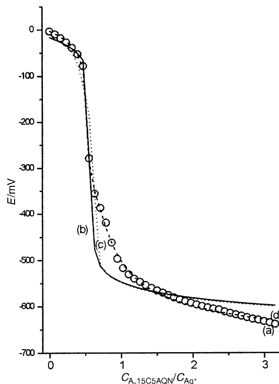
Fig. 6 Potentiometric measurement of silver(i) perchlorate ( 6.00 \times 10^{-4} \text{ mol dm}^{-3} ) with \text{A}_2\text{-15C5AQN 8} ( 0\text{--}2.00 \times 10^{-3} \text{ mol dm}^{-3} ) as a function of molar ratio C_{\text{A}_2\text{-15C5AQN}}/C_{\text{Ag}^+} . The experimental points are (a) (open circles) and the fitting curves for the models are 1 (b) (line), 4 (c) (dotted line), 8 (d) (dashed line).
